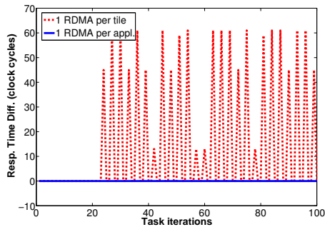
Figure 3: JPEG, vld response time difference ( JPEG-multi - JPEG-single )
