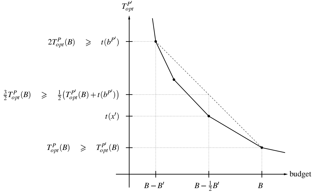
Figure 2: The convexity of T_{opt}^{P'} yields t(x') \leq \lceil \frac{3}{2} T_{opt}^P(B) \rceil .
